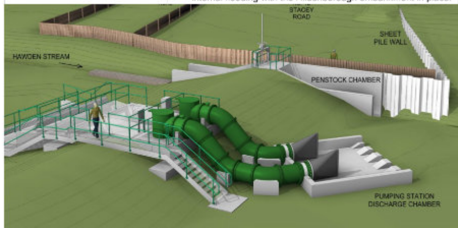
Above: Indicative design of the Hildenborough scheme
